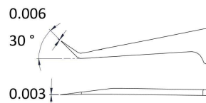
Dimensions inch
